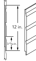
TWELVEFOUR COTTAGE LAP 7/8 in. GROOVE 1/2 in. LAP SIDING
