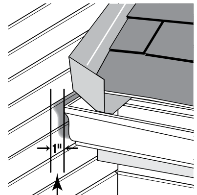
1 in. clearance between gutter end and siding
