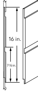
CHANNEL RUSTIC 1 in. GROOVE 1/2 in. LAP SIDING
