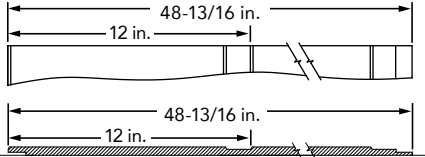
7/16 in. OLD MILL® 12 in. REVERSE BOARD AND BATTEN - 1-3/16 in. GROOVE
