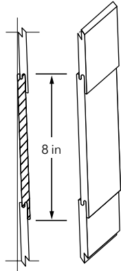
8 in SURE LOCK 1/2 in LAP SIDING
