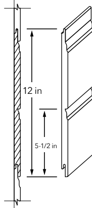
SURE LOCK SIX COTTAGE LAP 7/8 in GROOVE 1/2 in LAP SIDING
